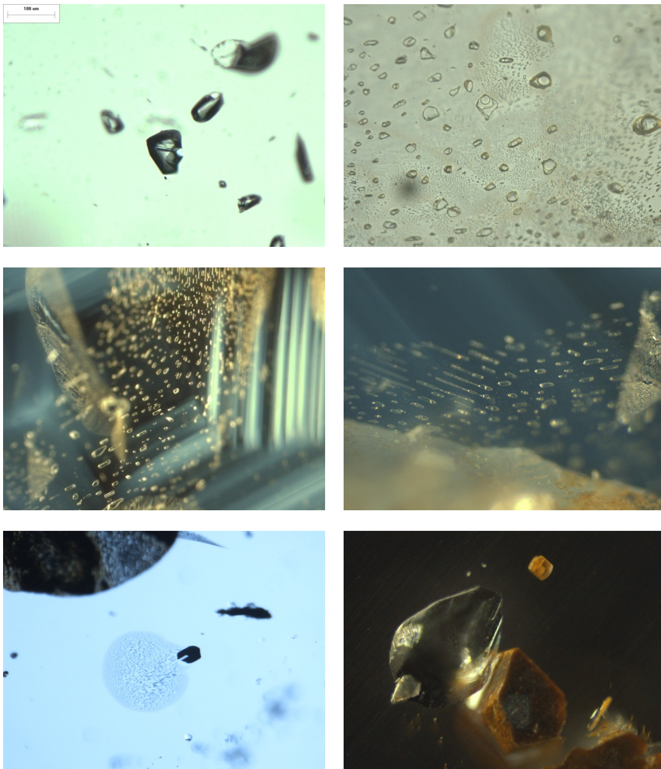
Figure 36. Top left: cavity filled with CO 2 liquid, vapor, diaspore crystal and unknown crystal 400x. Top right: multi phase primary inclusions containing mixture of CO 2 liquid and vapor, another liquid, and diaspore crystals. Middle: multi phase primary inclusions in the foreground following the trigonal symmetry of the sapphire, in the background a secondary fluid inclusion “fingerprint” 400x. Bottom: a single primary negative cavity containing diaspore crystal with partially healed “fingerprint”. Primary inclusions with iron staining showing bipyramidal habit.
