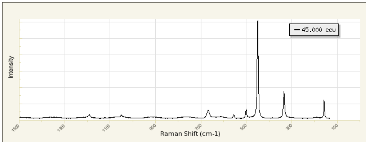
Figure 38. Diaspore Raman spectrum from RRUFF Database specimen ID: R060287
