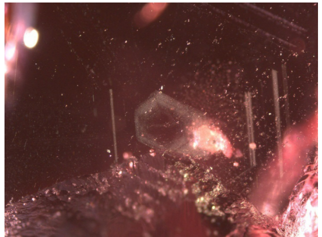
Figure 6. Exsolved rutile needles at 20x and again at 50x using oblique and darkfield illumination and microscopic rutile particles following hexagonal symmetry.
