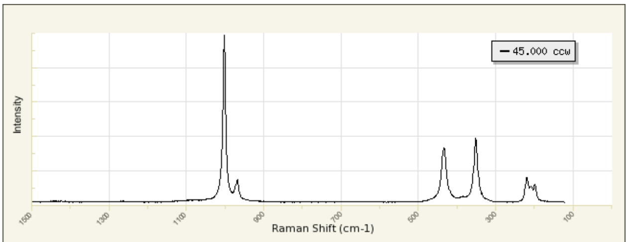
Figure 11. Zircon Raman spectrum from RRUFF Database, Specimen ID: R050034.
