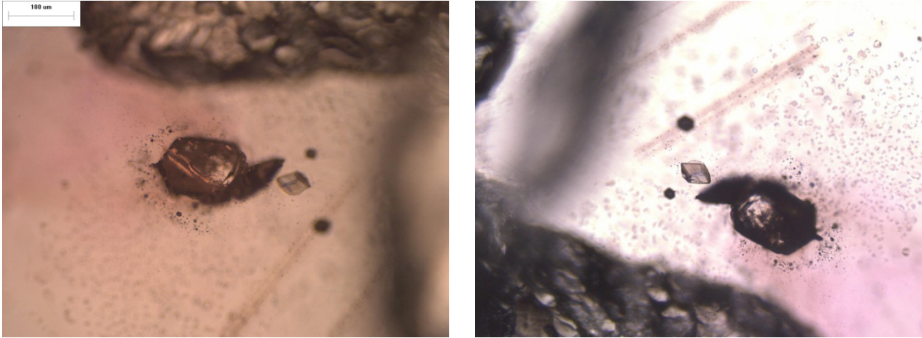
Figure 30. Corroded muscovite crystal with two well-formed hexagonal muscovite platelets and unknown rhombohedral crystal. 100x bright-field illumination.
