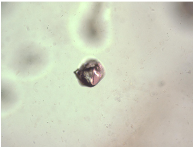
Figure 33. Top: Fluorite and calcite crystals, 50x and 100x. Bottom left: Fluorite octahedral in front with rounded, semi corroded calcite crystal attached at back. Bottom right: Corroded calcite crystal with fluorite crystal attached on right. 200x.
