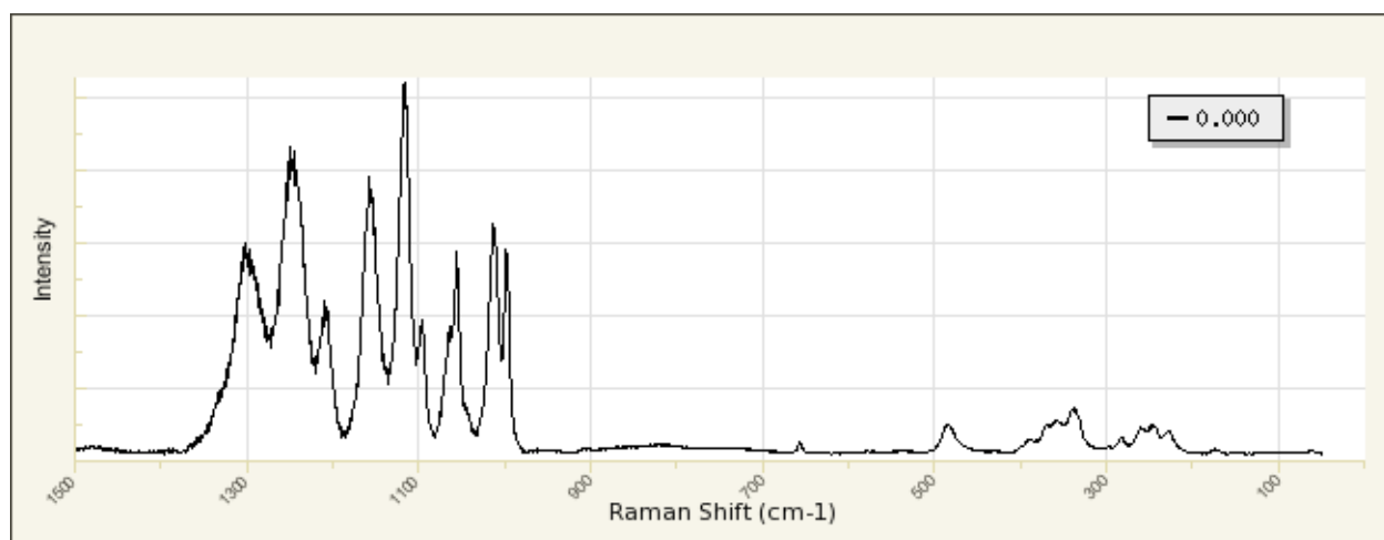
Figure 16. Xenotime Raman spectrum from RRUFF Database specimen ID: R050178.
