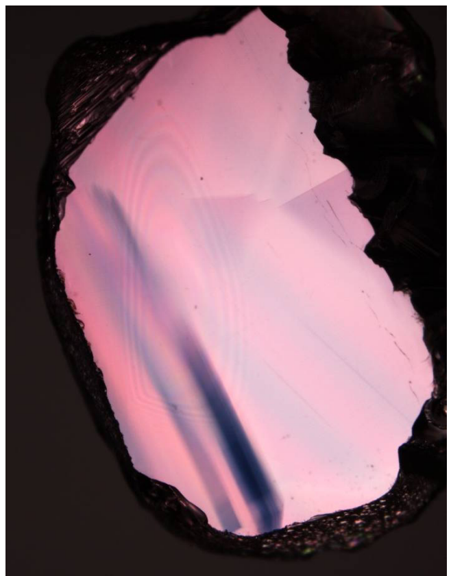
Figure 39. Blue growth zoning mirrors internal distribution of external crystal faces, basal pinacoid, rhombohedra, and various bipyramid forms can be recognized 20x light field illumination. Blue and pink zoning following internal crystal faces 20x.
