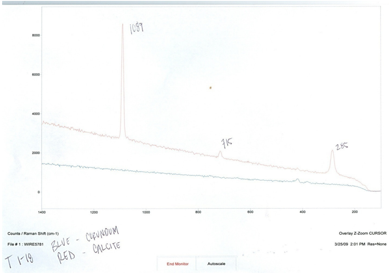
Figure 21. Calcite Raman spectrum with host corundum spectrum below.
