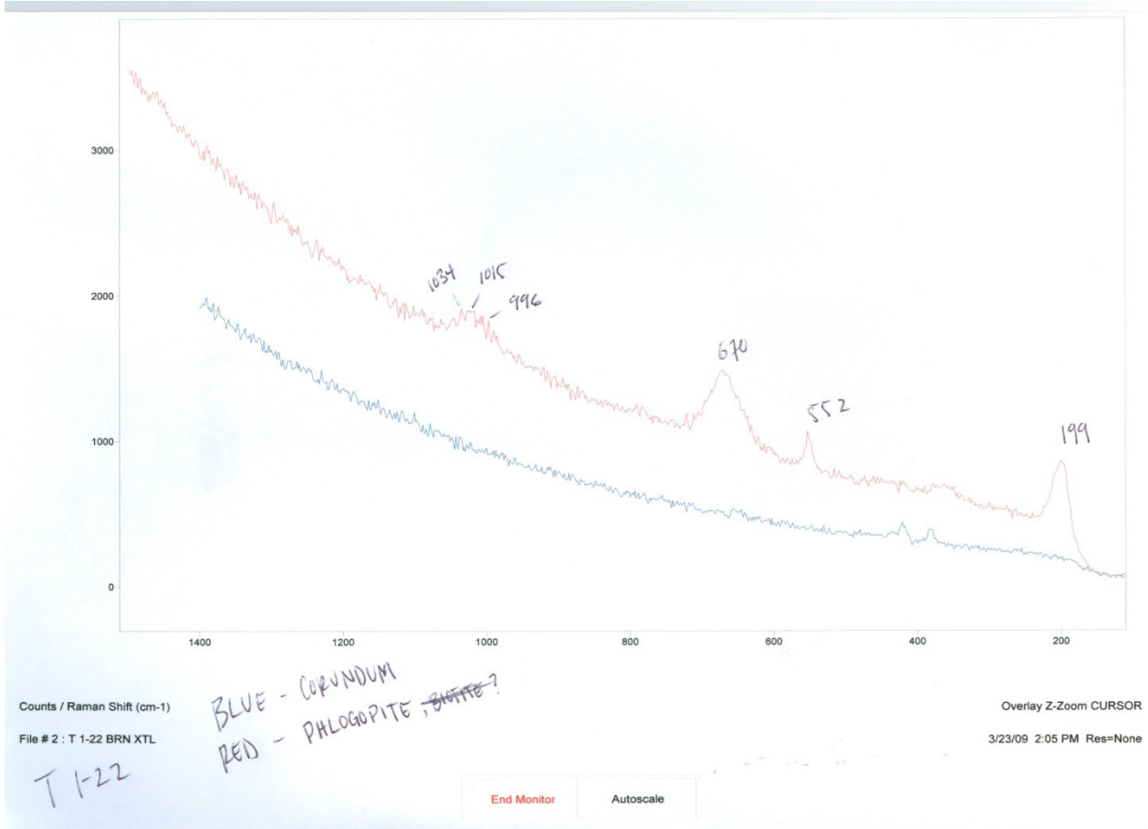
Figure 13. Phlogopite Raman spectrum with host corundum spectrum below..
