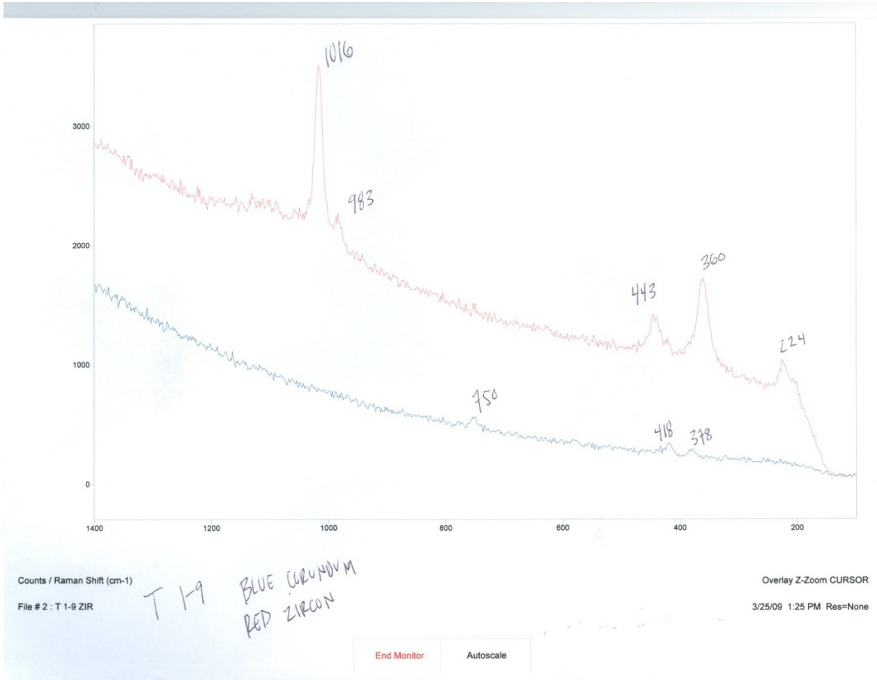
Figure 10. Zircon Raman spectrum, with the host corundum spectrum below.
