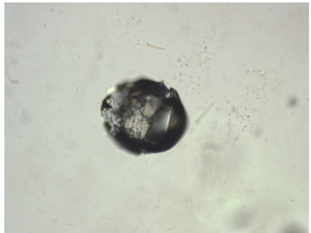
Figure 33. Top: Fluorite and calcite crystals, 50x and 100x. Bottom left: Fluorite octahedral in front with rounded, semi corroded calcite crystal attached at back. Bottom right: Corroded calcite crystal with fluorite crystal attached on right. 200x.
