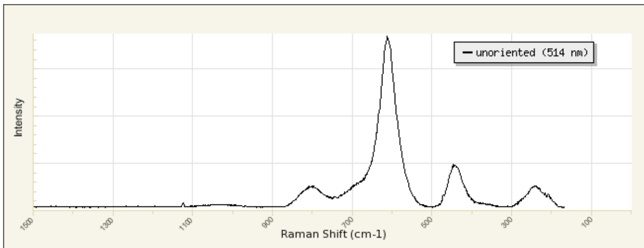
Figure 8. Rutile raman spectrum from specimen ID: R040049 RRUFF Database.
