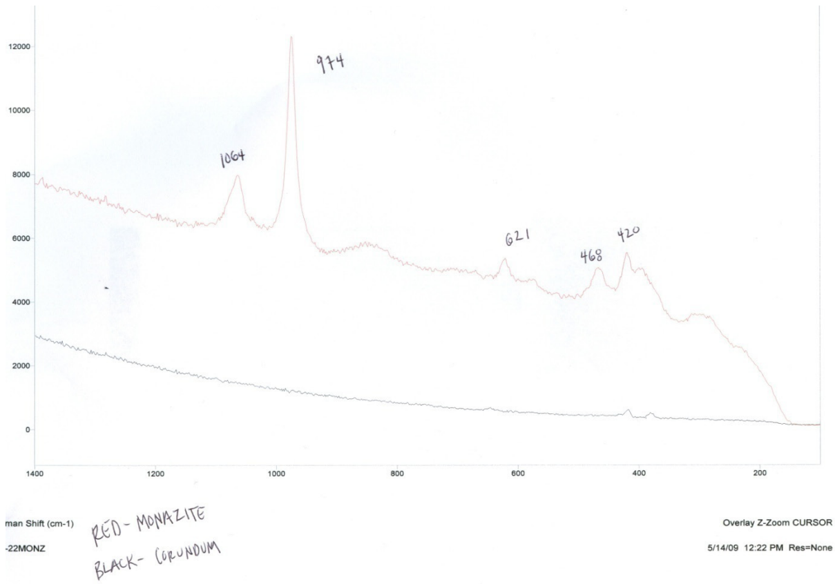
Figure 17. Raman spectrum of monazite over spectrum of host corundum.
