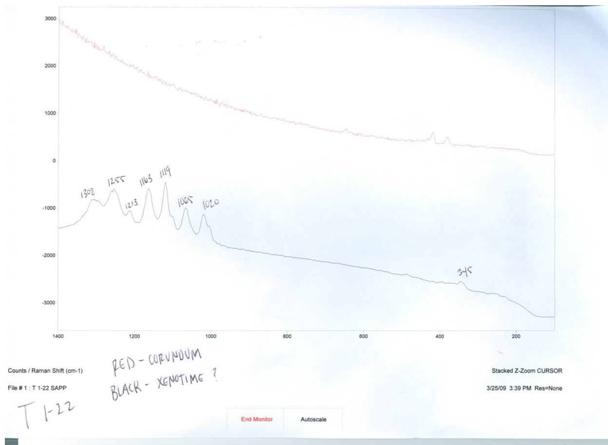
Figure 15. Xenotime Raman spectrum with host corundum spectrum above.
