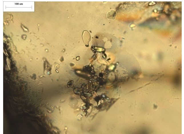
Figure 12. Top: Brown phlogopite crystals. Bottom: Golden-brown tabular monazite crystals surrounded by clusters of zircons, phlogopite and xenotime. 200x.
