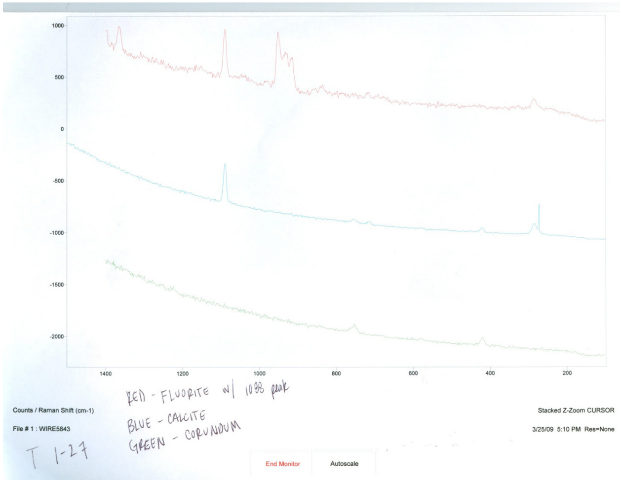
Figure 34. Raman spectra from fluorite octahedron attached to calcite crystal.
