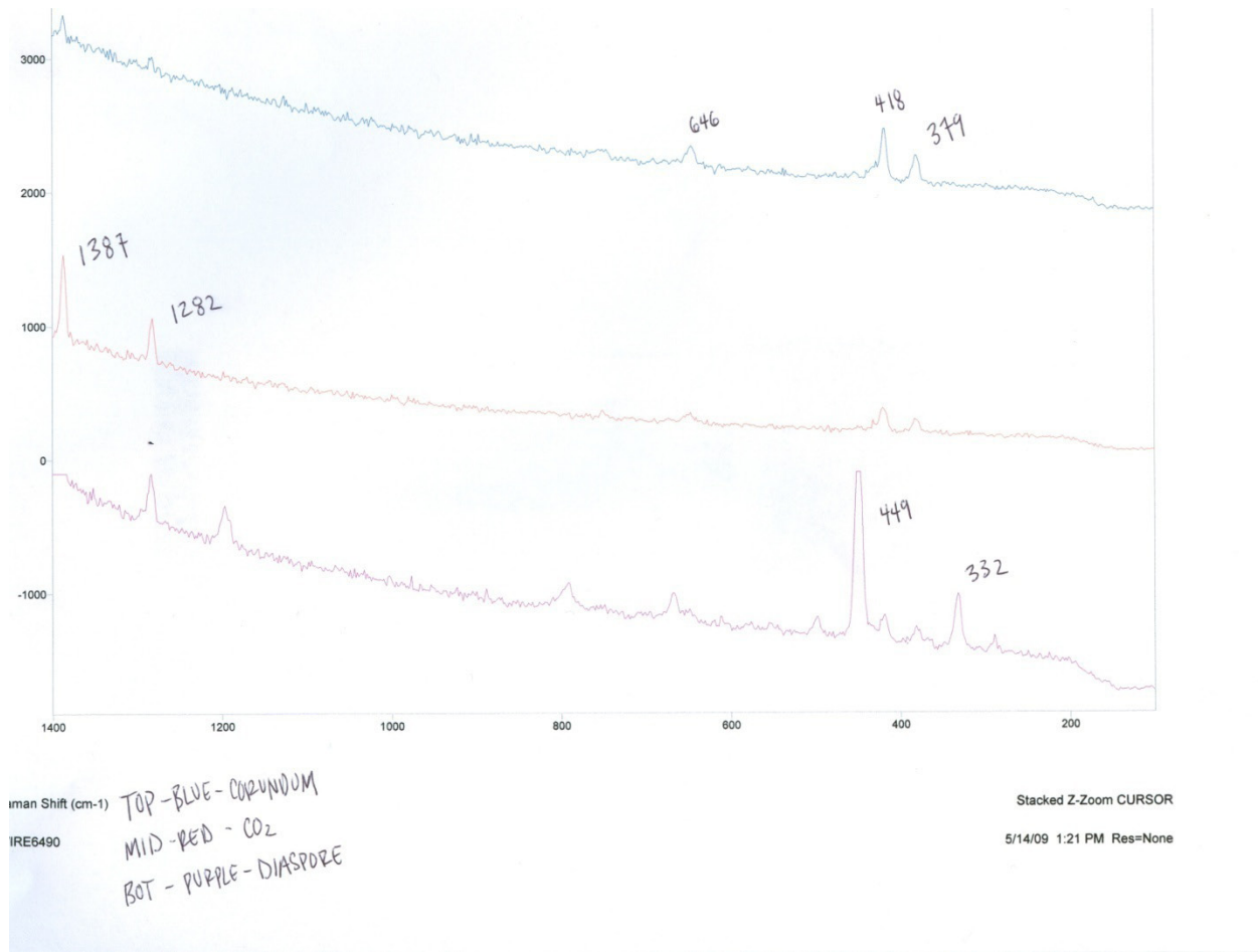
Figure 37. Top: Host corundum Raman spectrum, middle CO 2 Raman spectrum, bottom diaspore Raman spectrum.
