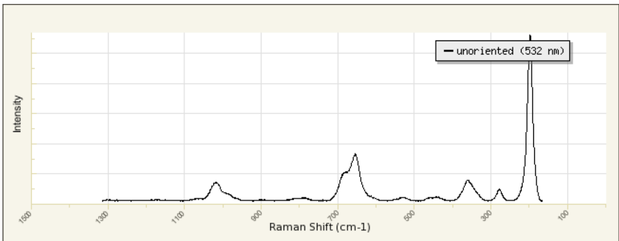
Figure 14. Phlogopite Raman spectrum from RRUFF Database specimen ID: R040144.
