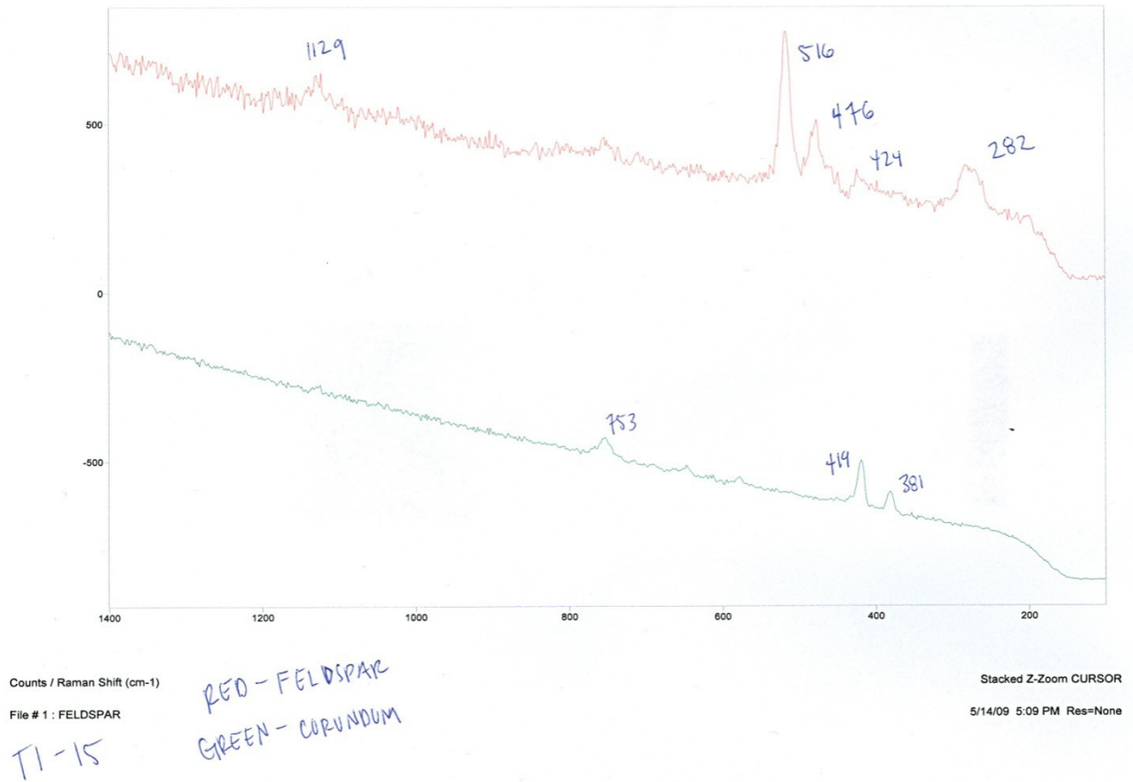
Figure 28. Feldspar raman spectra with host corundum spectra below.
