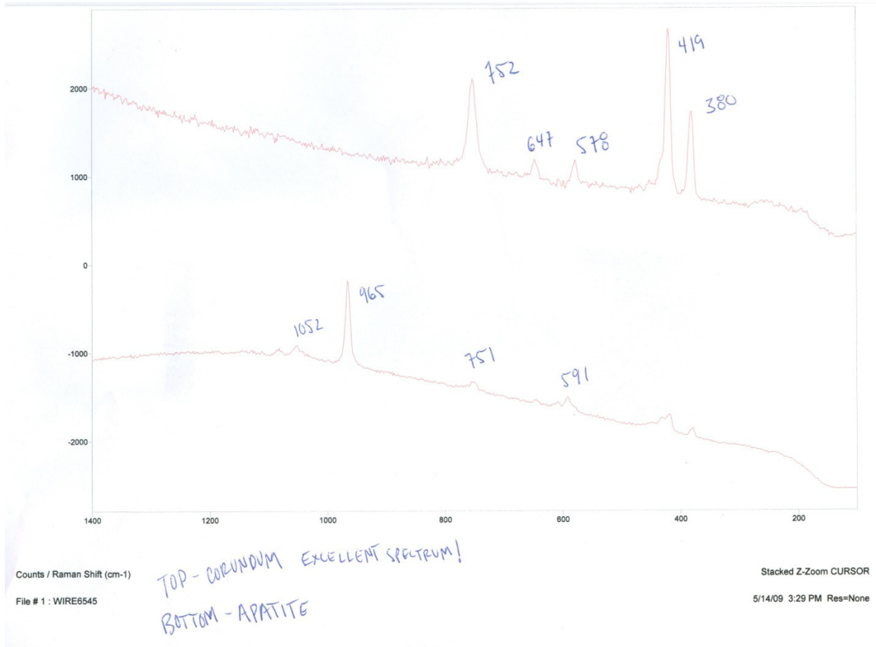
Figure 25. Apatite Raman spectrum with host corundum spectrum above.
