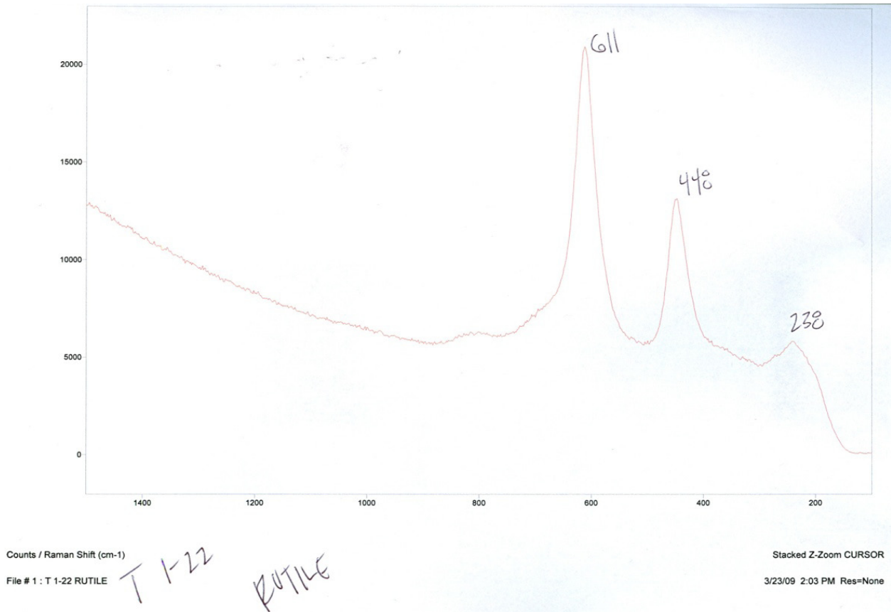
Figure 7. Raman spectra of rutile showing characteristic Raman peaks.
